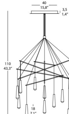
MIKADO LA 6 GLASS_S 6x3,1W 1950 Lm 3000K Cri>80 220-240V LED CE F IP 20 3
