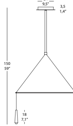
MIKADO S2L GLASS_L 2x3,1W 650 Lm 3000K Cri>80 220-240V LED CE F IP 20 3
