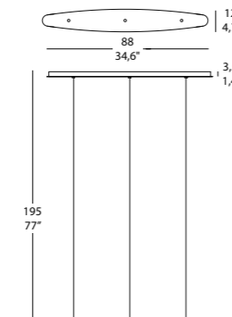
MIKADO S2L GLASS_L 2x3,1W 650 Lm 3000K Cri>80 220-240V LED CE F IP 20 3
