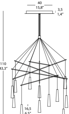
MIKADO LA 6_S 6x3,1W 1950 Lm 3000K Cri>80 220-240V LED CE F IP 20 3
