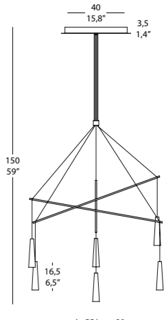
MIKADO LA 6_L 6x3,1W 1950 Lm 3000K Cri>80 220-240V LED CE F IP 20 3
