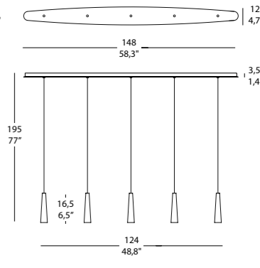
MIKADO SSL_L 5x3,1W 1625 Lm 3000K Cri>80 220-240V LED CE F IP 20 3
