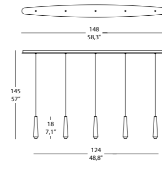
MIKADO SSL GLASS_S 5x3,1W 1625 Lm 3000K Cri>80 220-240V LED CE F IP 20 3
