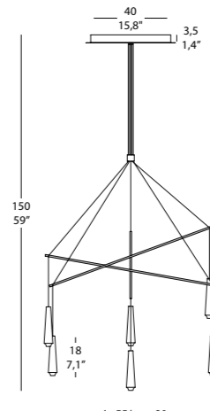
MIKADO LA 6 GLASS_L 6x3,1W 1950 Lm 3000K Cri>80 220-240V LED CE F IP 20 3
