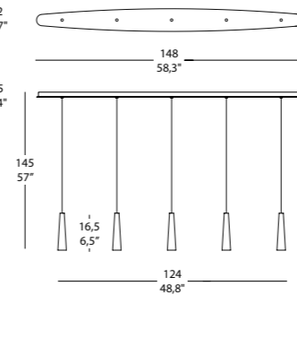
MIKADO SSL_S 5x3,1W 1625 Lm 3000K Cri>80 220-240V LED CE F IP 20 3
