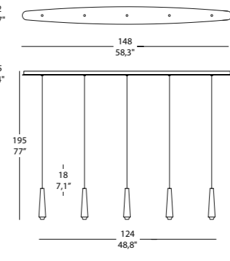
MIKADO SSL GLASS_L 5x3,1W 1625 Lm 3000K Cri>80 220-240V LED CE F IP 20 3
