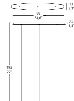
MIKADO S2L_L 2x3,1W 650 Lm 3000K Cri>80 220-240V LED CE F IP 20 3
